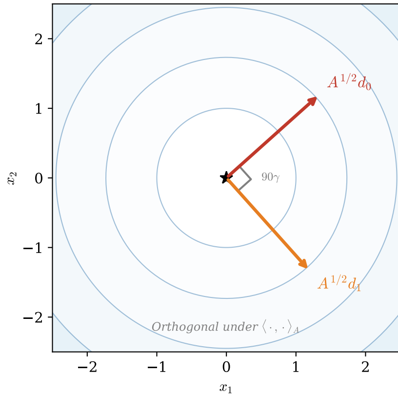
A^{1/2} -Transformed Space
